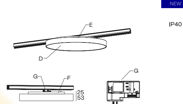
3. TRACKLIGHT \varnothing 250 mm to \varnothing 650 mm
