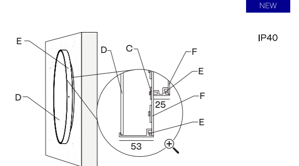
4. WALL SURFACE \varnothing 250 mm to \varnothing 650 mm
